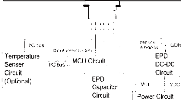
Driver PCBA
